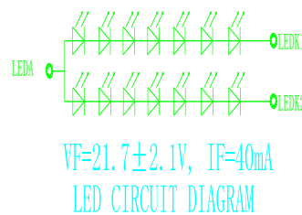
Fig.2*Schematics drawing of lighting (绘制照明图 图.2)
